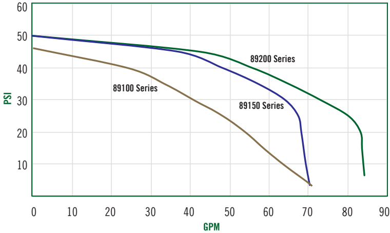
Flow GPM vs. Pressure PSI Curve
